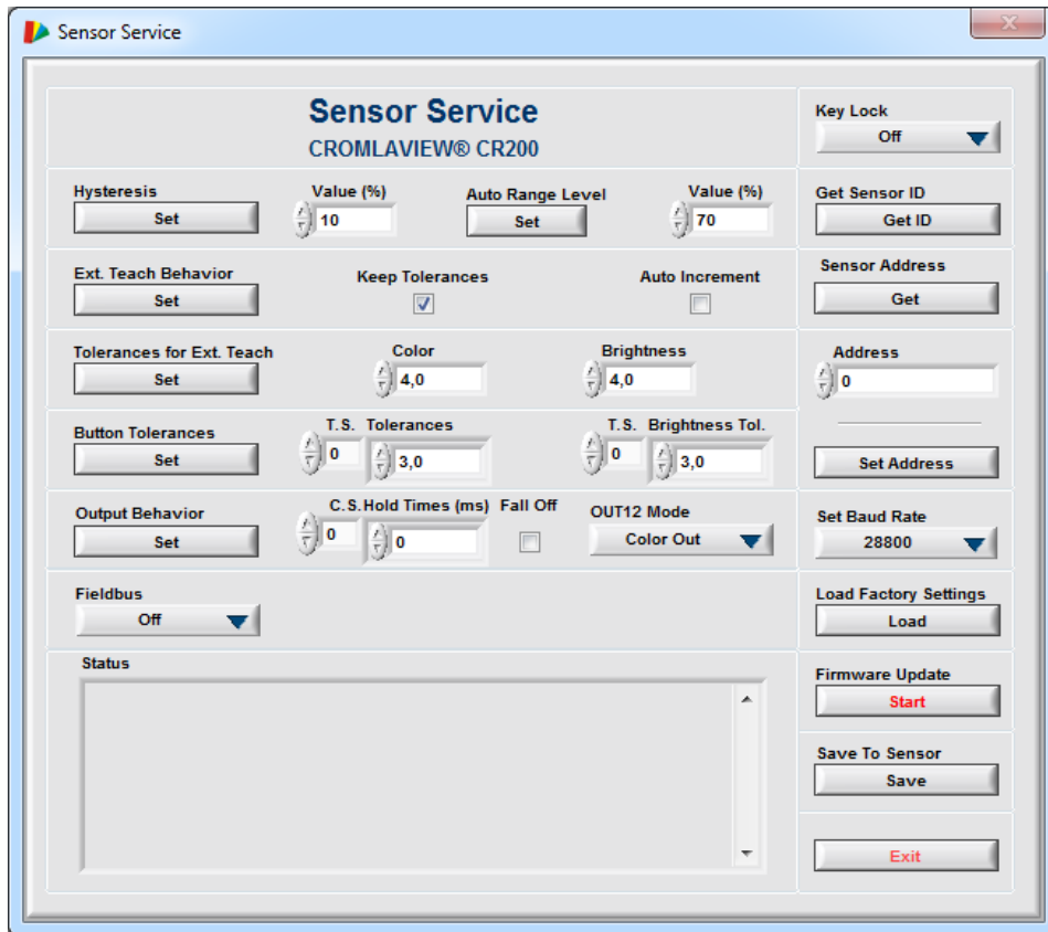
Fig. 16: “Sensor Service” program window
