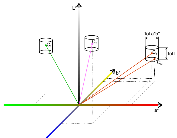
Fig. 7: Diagram for explaining the recognition mode “Check Cylinder.”
