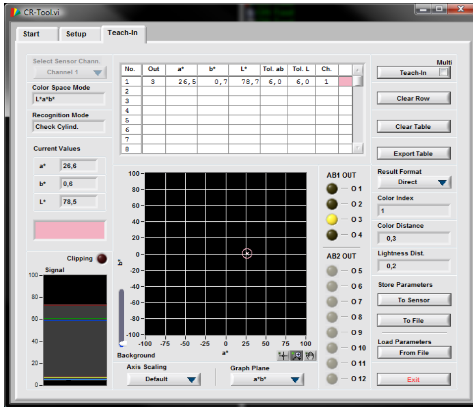
Fig. 12: Teach-In window for teaching colors and displaying recognition results
