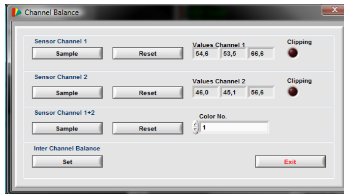
Fig. 10: Inter-channel balance window
